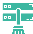
Data Cleaning
